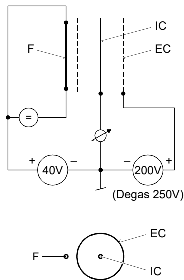
Diagram of the BA measuring system
