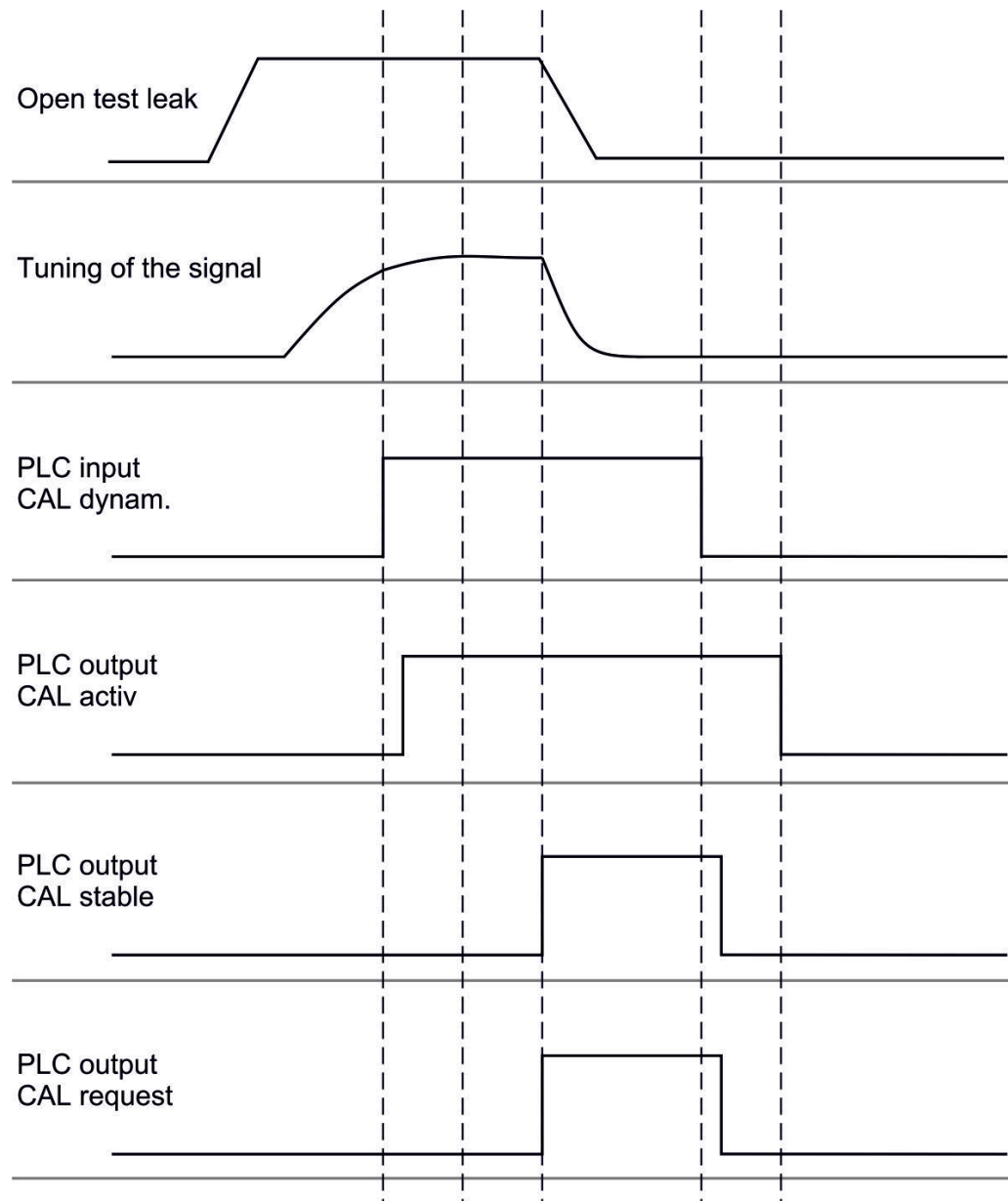
Fig. 7: Fig. 7 External dynamic calibration with IO1000 using the example of sniffer line SL3000XL, description of PLC inputs and outputs: "Assigning inputs and outputs [► 57]"
