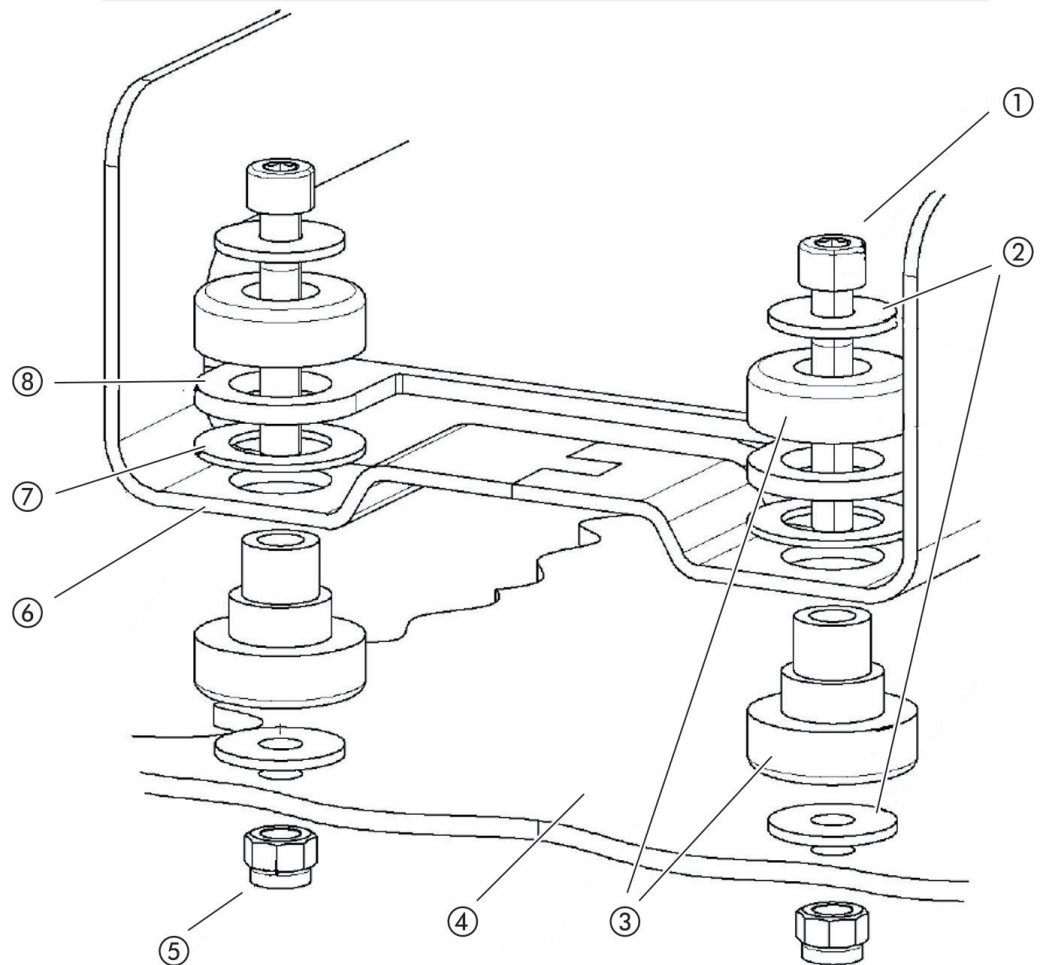
Fig. 5: Components of a fastener
