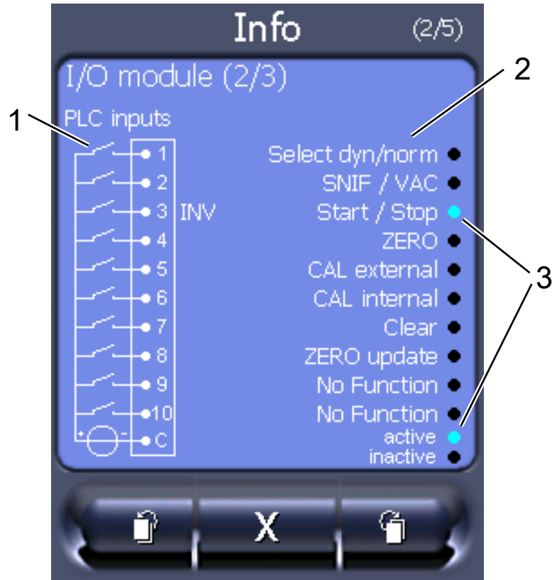
Fig. 12: I/O module (2): Visualized information to the digital inputs
