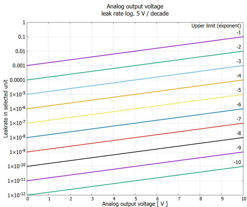
Fig. 10: Analog output voltage leak rate log. 5 V / decade
