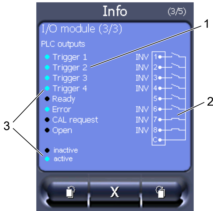
Fig. 13: Visualized information to the digital outputs
