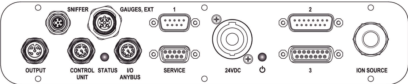
Fig. 3: MSB box connections
