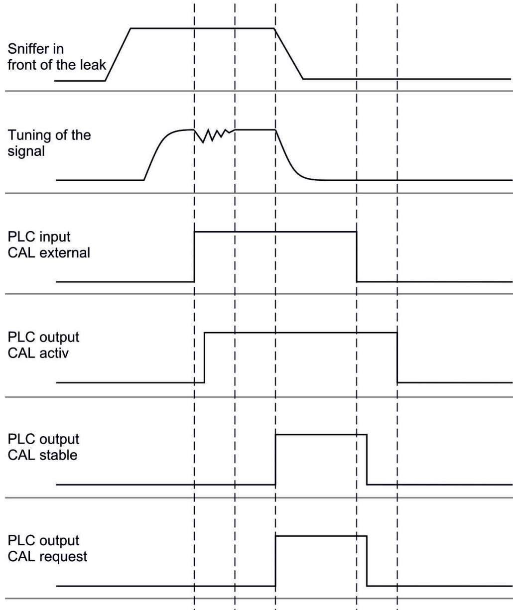
Fig. 6: External calibration with IO1000 using the example of sniffer line SL3000XL, description of PLC inputs and outputs: "Assigning inputs and outputs [► 57]"
