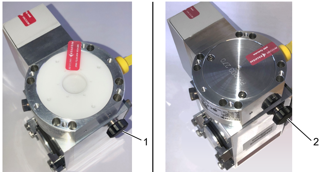
Fig. 17: Turbo molecular pump SplitFlow 80 with different covers
