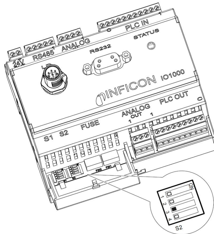
Fig. 16: DIP switch on the I/O module
