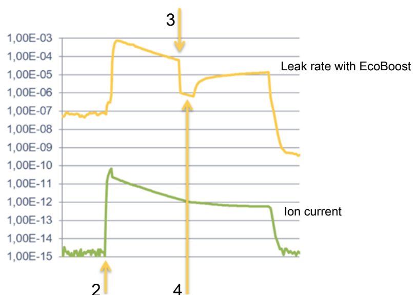
Fig. 8: Example of measurement curves (EcoBoost)
