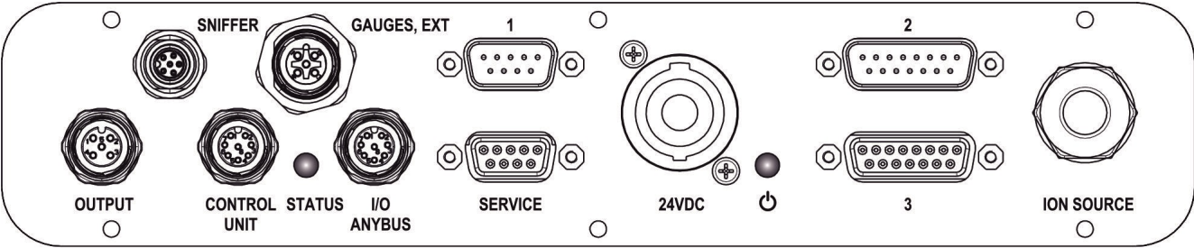
Fig. 6: Connessioni box MSB
