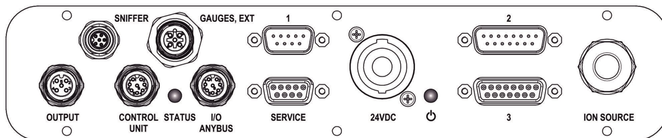
Abb. 6: Anschlüsse MSB-Box
