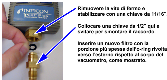
Figura 7. Raccordo Pilot Plus
