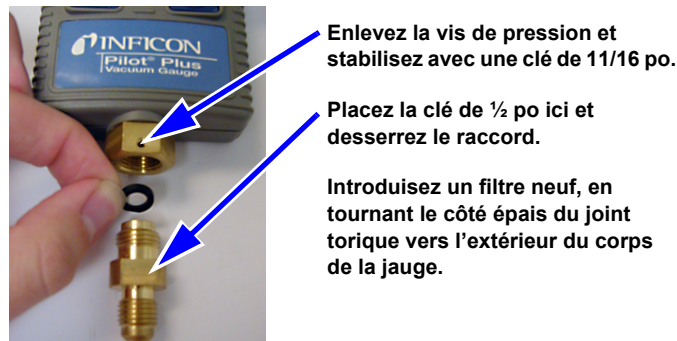
Figure 6. Raccord Pilot Plus
